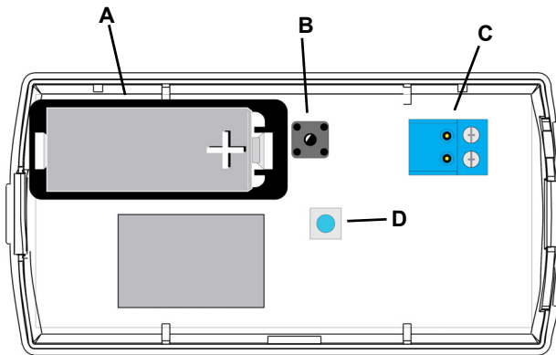
Figure 1 EN1501/EN1501-XL Components
